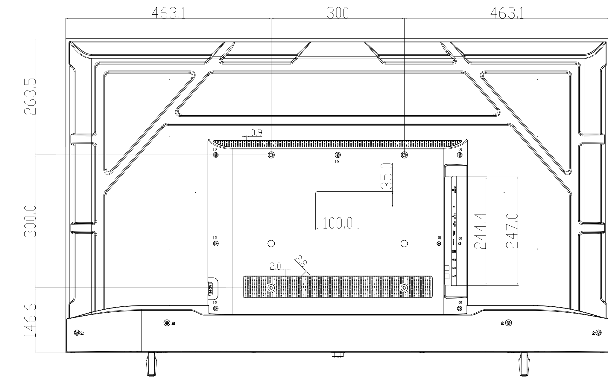
(BACK VIEW)
