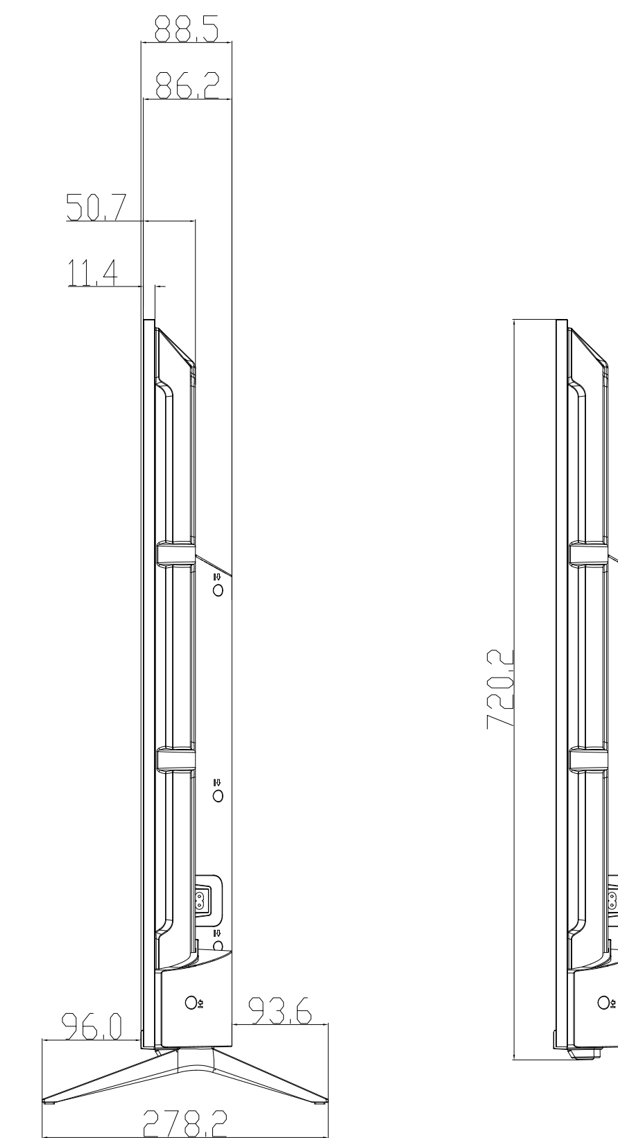
(RIGHT VIEW)
