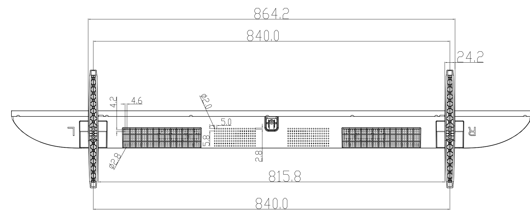
(BOTTOM VIEW)
