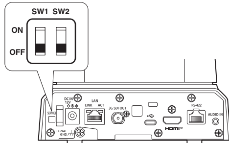
Service switch
