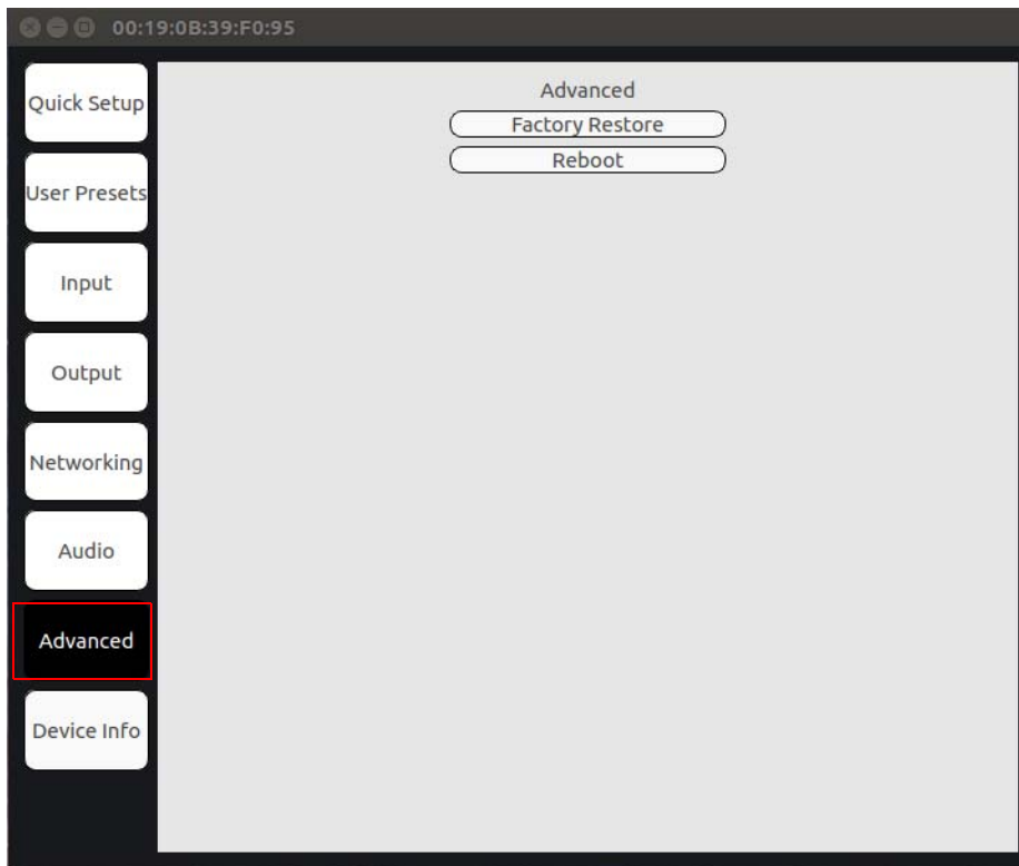
FIG. 18 Advanced Page
