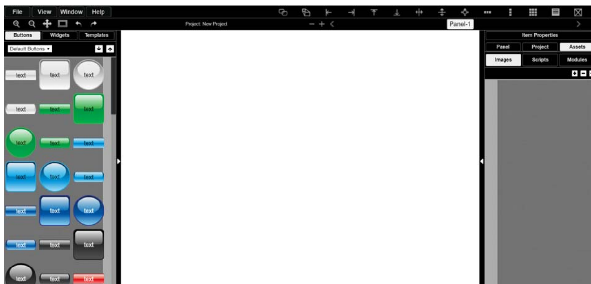
FIG. 45 Project Editor
